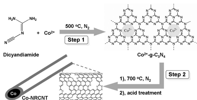
Figure 1. Synthesis of Co-NRCNTs: Step 1: thermal treatment at 500\text{ }^{\circ}\text{C} in \text{N}_2 atmosphere of a mixture of dicyandiamide and \text{CoCl}_2\cdot 6\text{H}_2\text{O} to form \text{Co}^{2+}\text{-g-C}_3\text{N}_4 . Step 2: additional thermal treatment at 700\text{ }^{\circ}\text{C} in \text{N}_2 atmosphere of the \text{Co}^{2+}\text{-g-C}_3\text{N}_4 , followed by acid treatment of the resulting material to etch away any accessible cobalt species on it.
